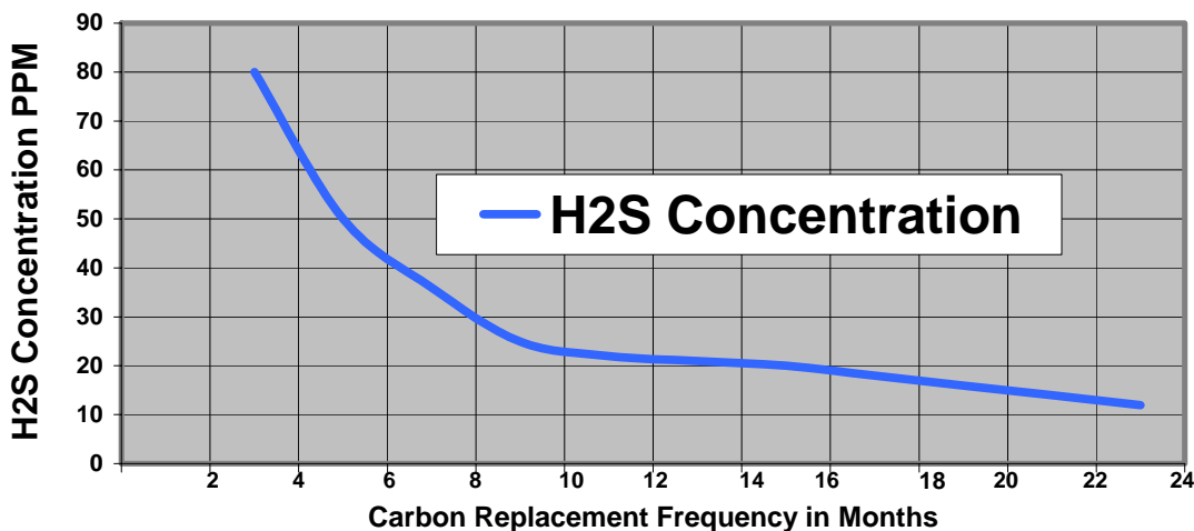
Estimated Life Expectancy of Activated Carbon. Based on 5CFM (Odorous Airflow)
